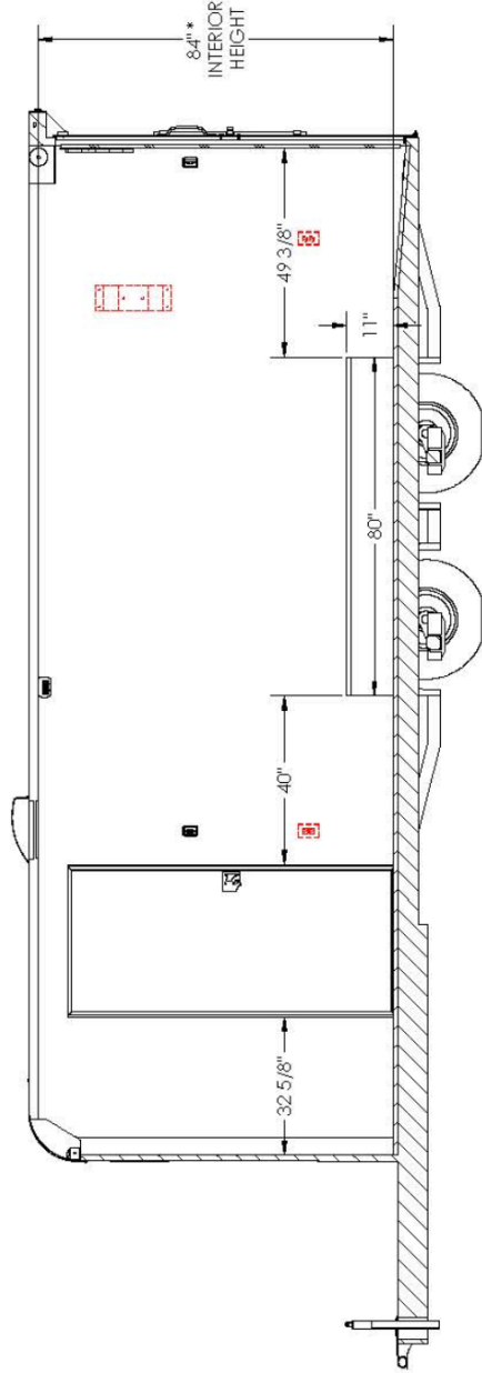
INTERIOR CURB SIDE SECTION B-B
